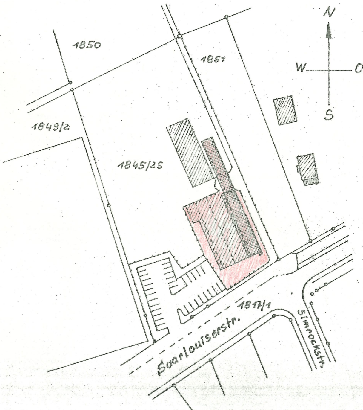
Lageplan M = 1:1000
